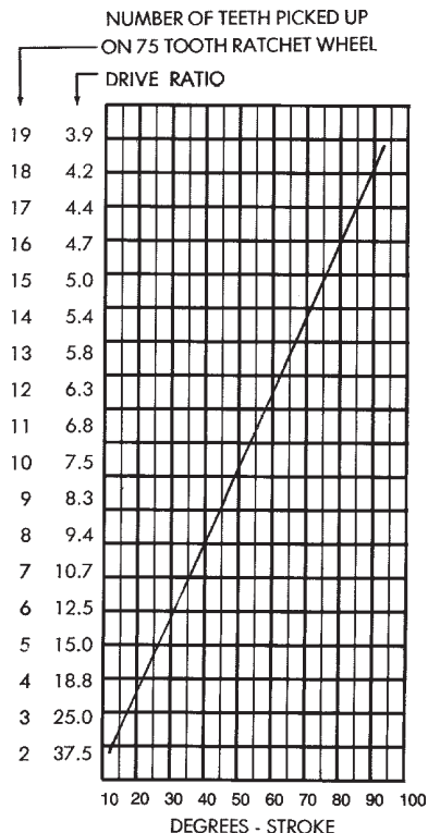
CHART: DRIVE RATIO PER DEGREE STROKE
